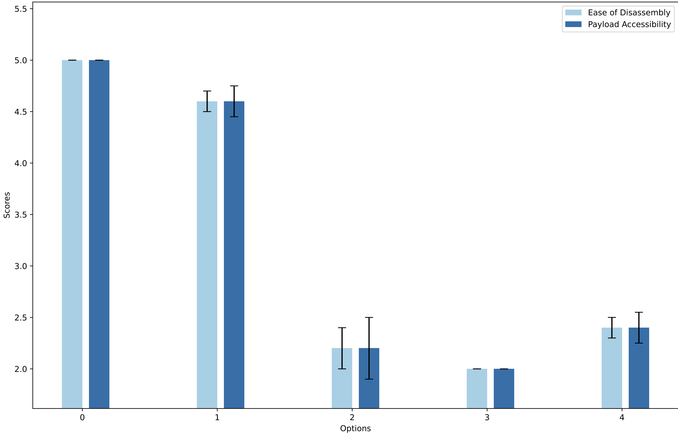
Combined KPI Sensitivity Analysis for Transportability
